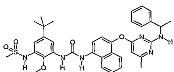
N-[5-tert-Butyl-2-methoxy-3-(3-{4-[6-methyl-2-(1-phenyl-ethylamino)-pyrimidin-4-yloxy]-naphthalen-1-yl}-ureido)-phenyl]-methanesulfonamide;
